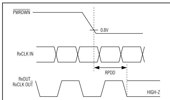
Figure 8. Power-Down Delay
